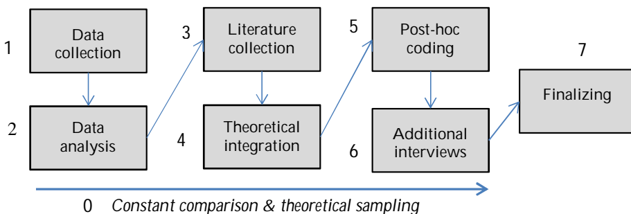
Figure 3 Research process
